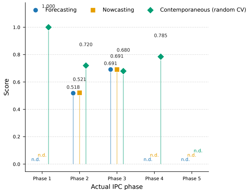
A Class-specific precision
