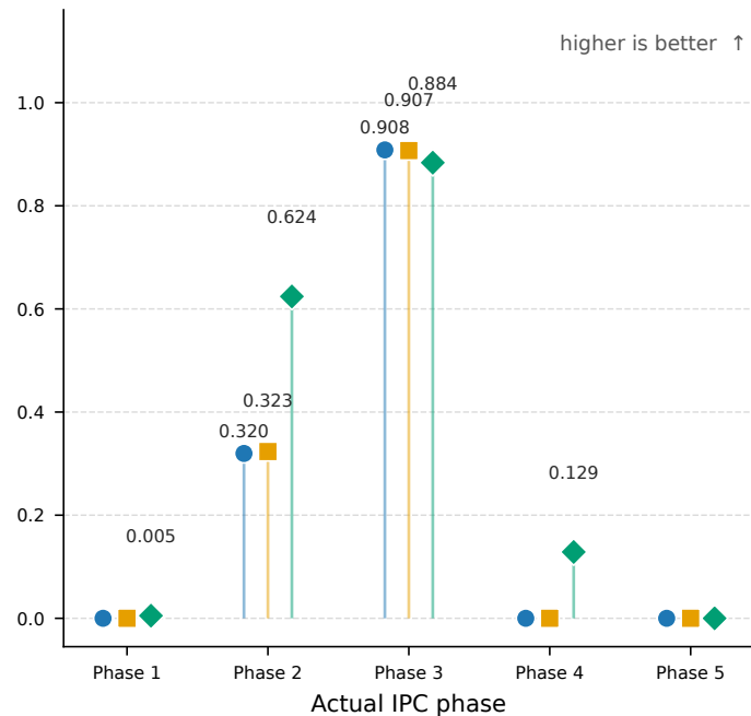
B Class-specific recall
